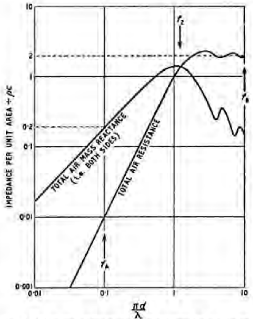
Fig. 3. Mass and radiation resistance curves for a circular diaphragm in a large baffle. The power radiated at any frequency f_1 well below f_2 is half that radiated at frequencies f_2 well above f_2 (see text).
